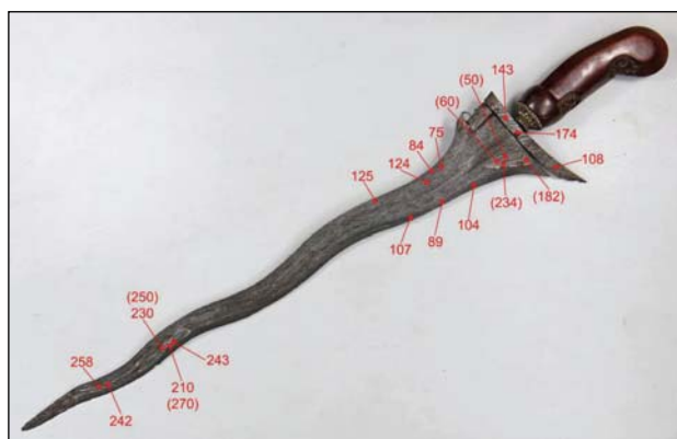
Figure 2: Photograph of kris N 32591, with locations and corresponding results of hardness measurements.
