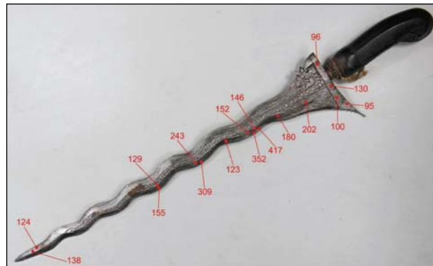
Figure 5: Photograph of kris MG 666, with locations and corresponding results of hardness measurements.
