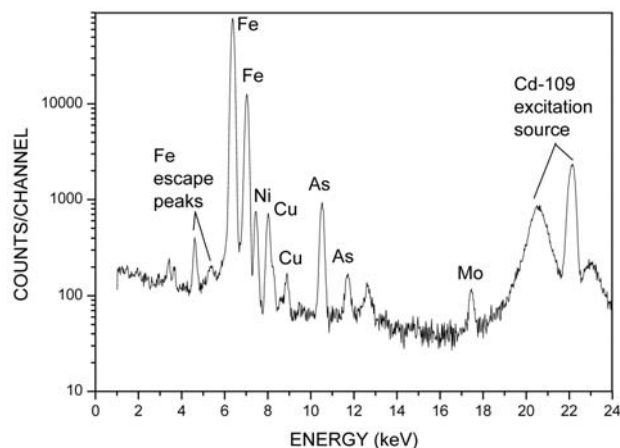
Figure 7. Fluorescence spectrum of a kris (N32591)
